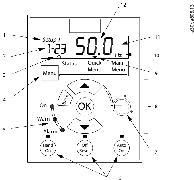
Illustration 7: Description of LCP Keys and Display
