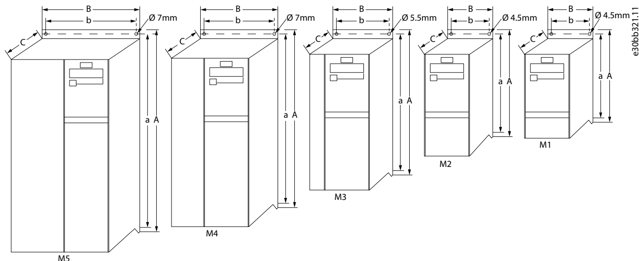
Illustration 1: Mechanical Dimensions
